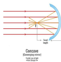
Concave mirror (Converging mirror)
